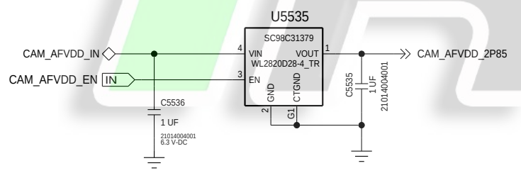
MAIN IMAGER AFVDD LDO 2.8V
