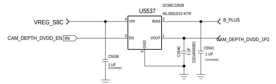
DEPTH DVDD LDO 1.2V
