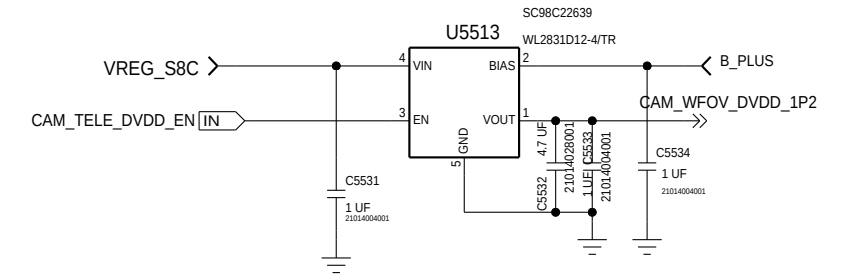
REAR WFOV IMAGER DVDD LDO 1.2V
