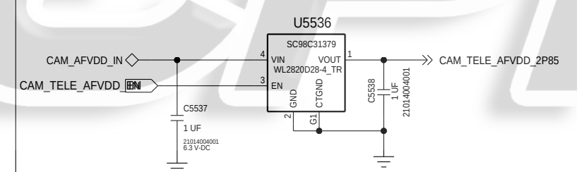
TELE AFVDD LDO 2.8V
