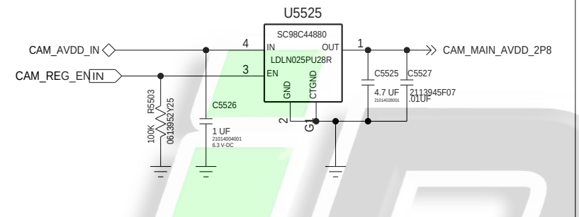
MAIN IMAGER AVDD LDO 2.8V
