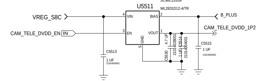
REAR TELE IMAGER DVDD LDO 1.2V
