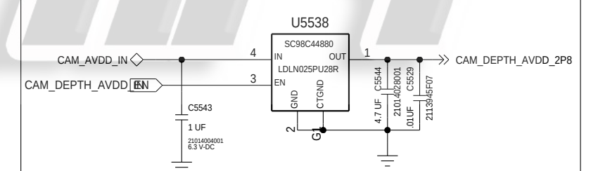
REAR DEPTH AVDD LDO 2.8V
