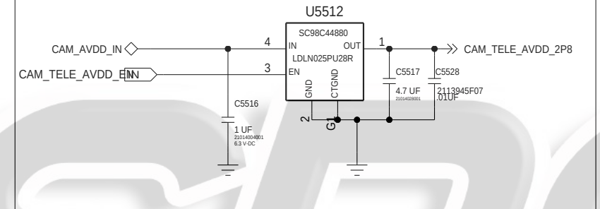
REAR TELE & WFOV AVDD LDO 2.8V
